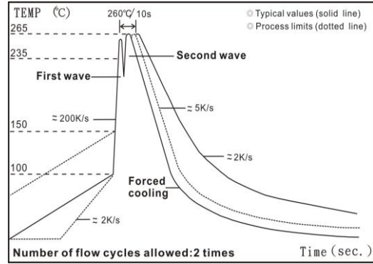
Wave Soldering (For R>10Ω)
